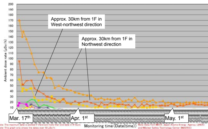
Fig. Trend on ambient dose rate monitoring at Monitoring post outside of 20km zone of 1F
